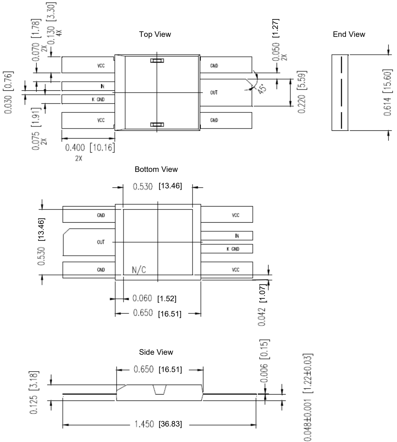
Fig. 23 Package Diagram
