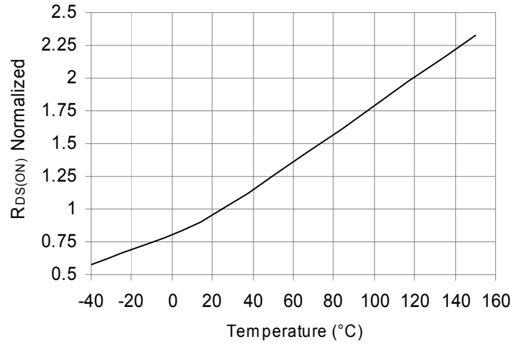
Normalized R_{DS(ON)} vs. Temperature I_D = 7.5A V_{GS} = 10V
